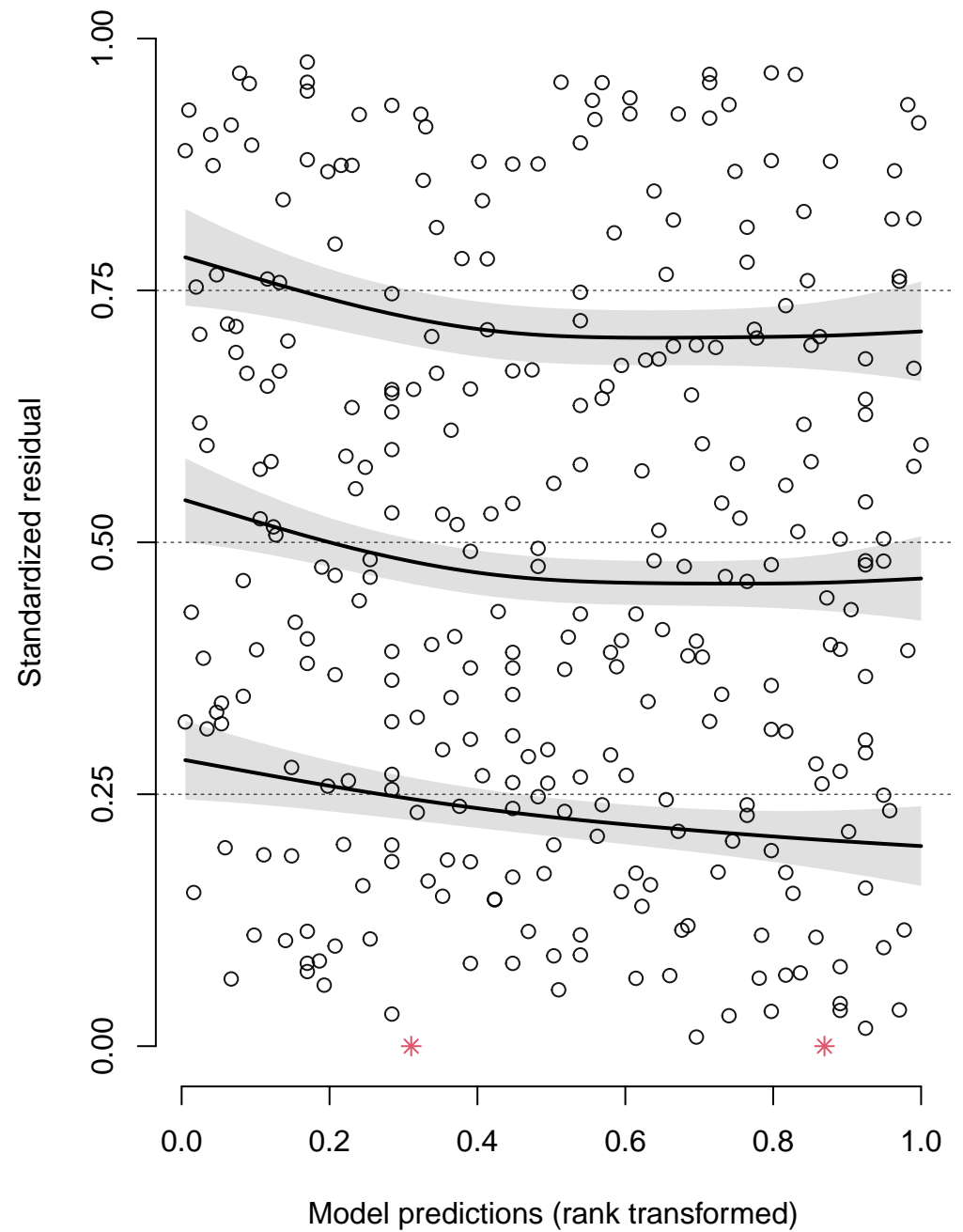
Residual vs. predicted No significant problems detected
