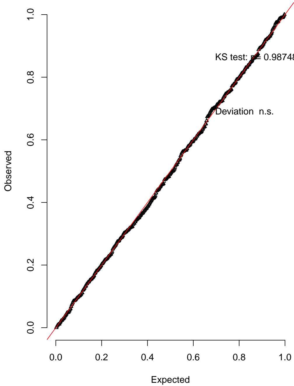
QQ plot residuals
