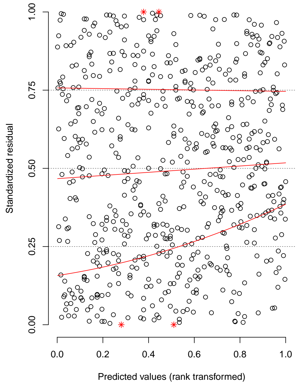
Residual vs. predicted lines should match
