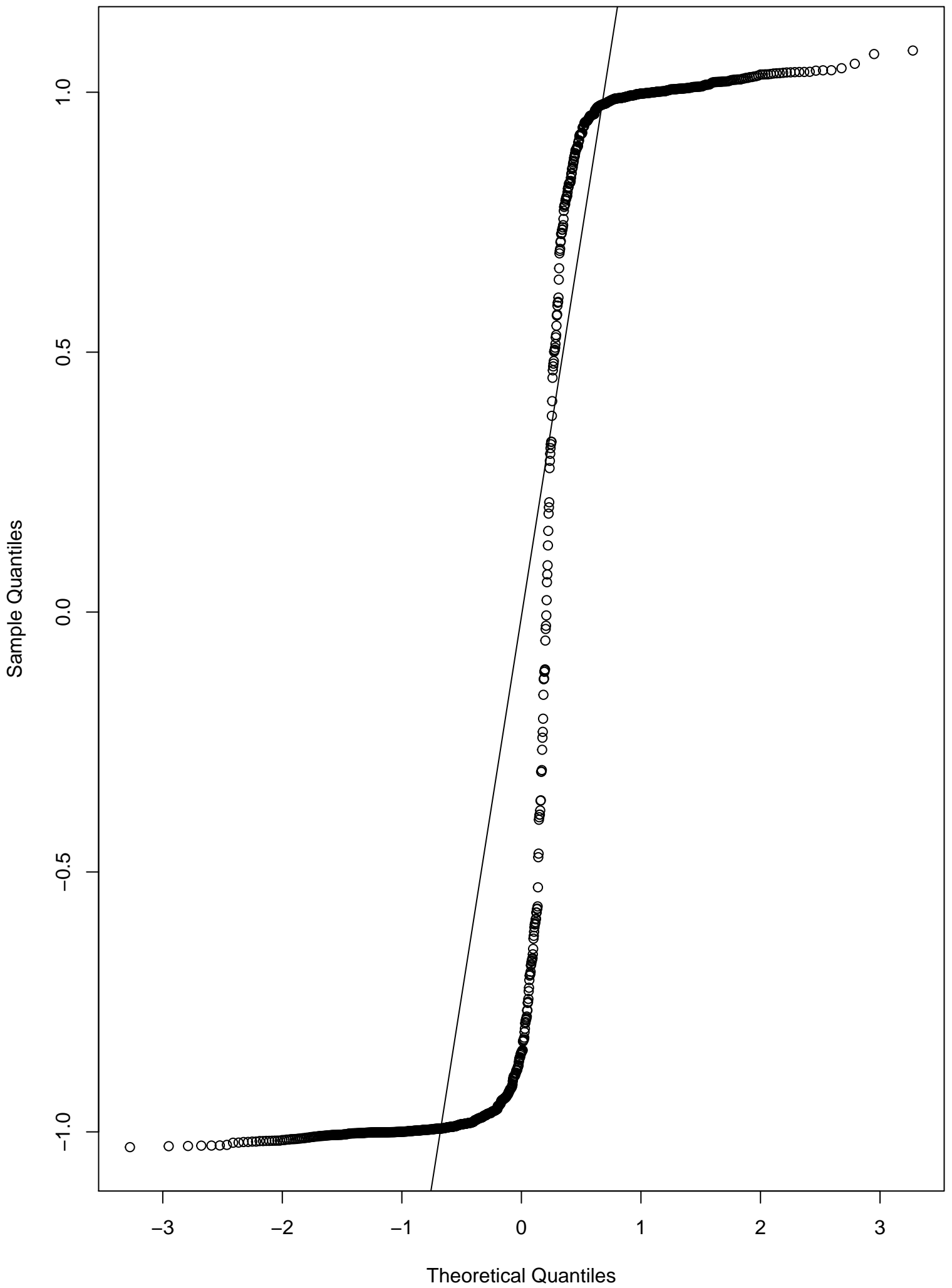
Normal Q-Q Plot
