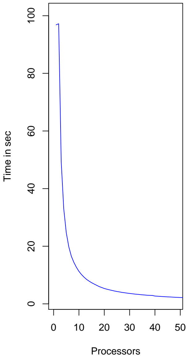
Bootstrap Benchmark
