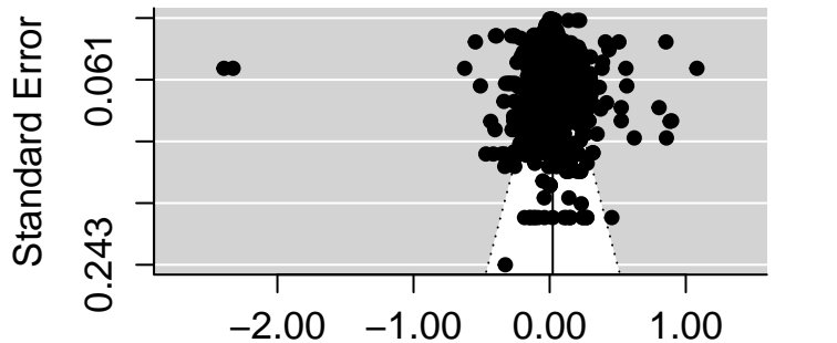
Funnel Plot
