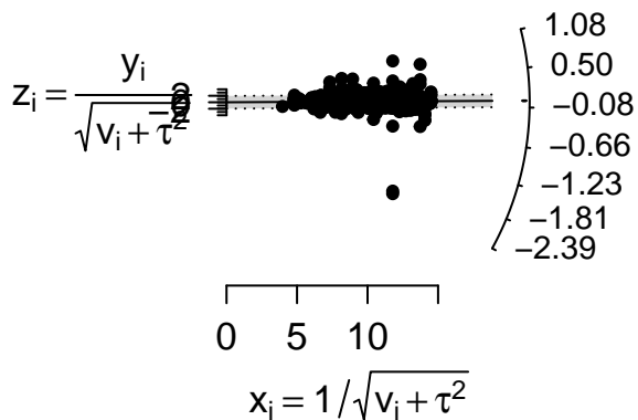
Radial Plot
