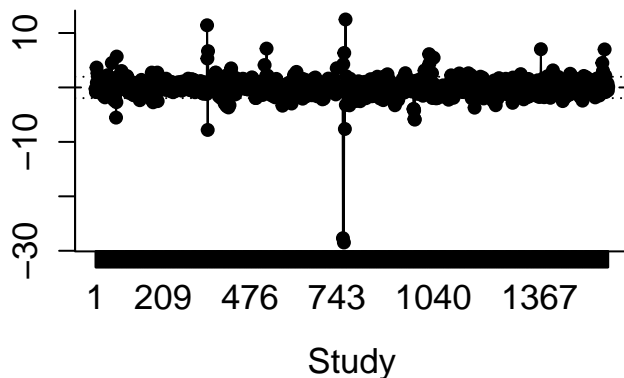
Standardized Residuals
