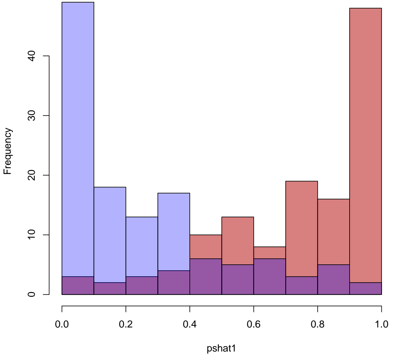
Histogram of pshat1
