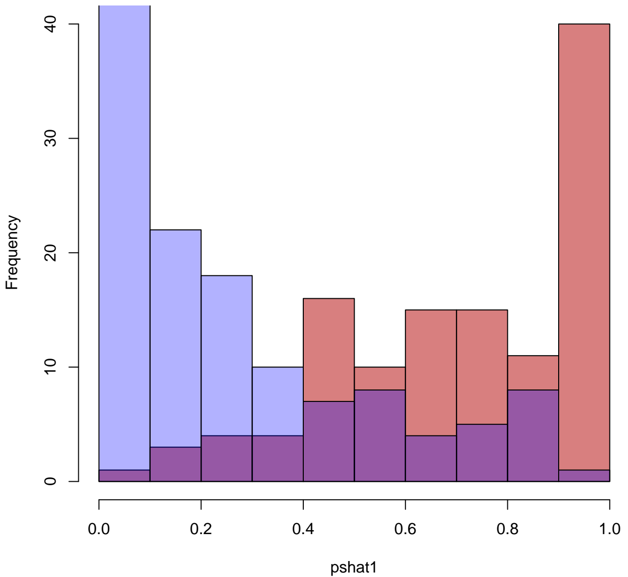
Histogram of pshat1
