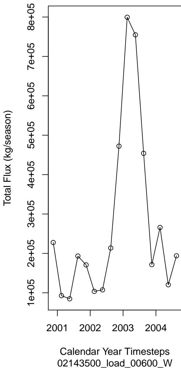
Fluxmaster versus EGRET/WRTDS Seasonal FLux Sum
