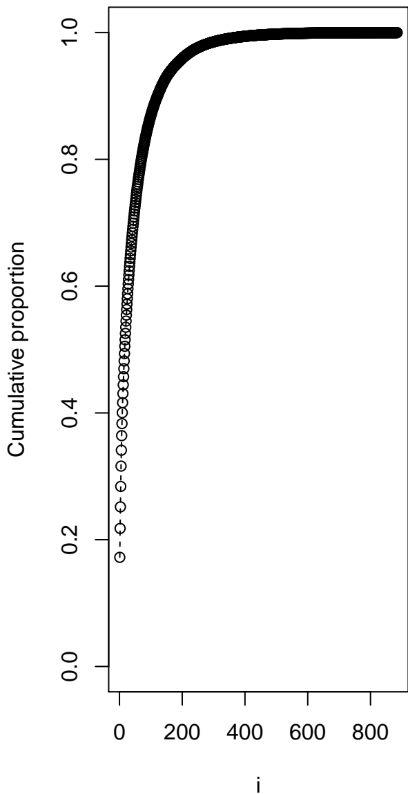
Proportion of total variance
