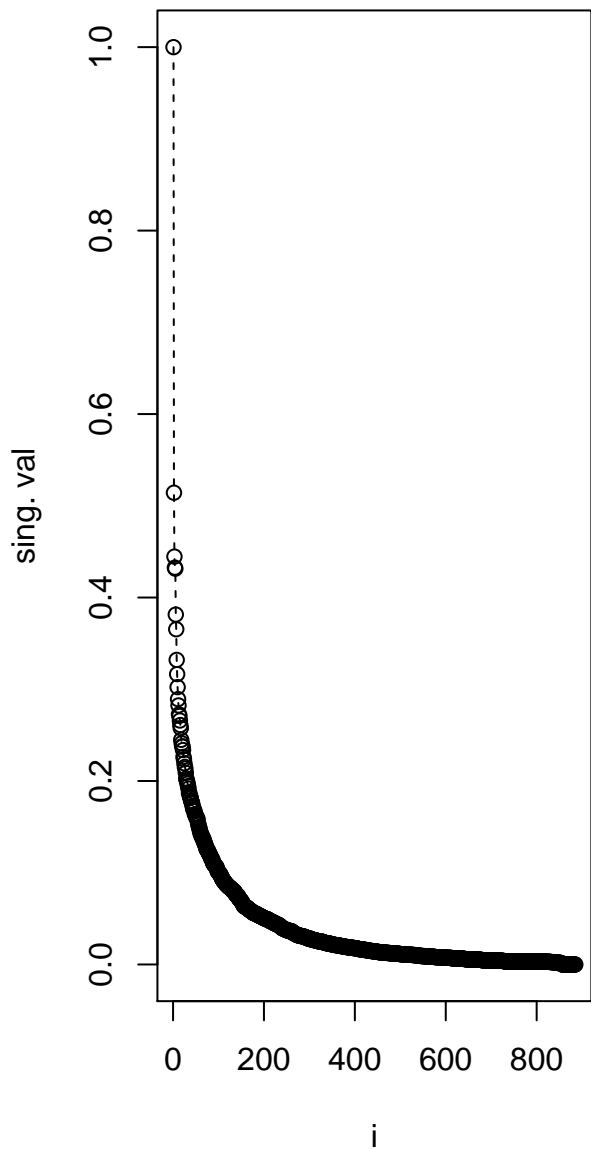
Standardized singular values
