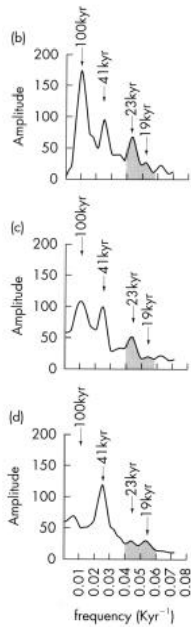
Figure 5.4 Spectral analysis of \delta^{18}\text{O} time series for the past two million years shows that periods characteristic of variations in eccentricity, obliquity and precession are all present in the oceanic record of fluctuations in the volume of land ice.
