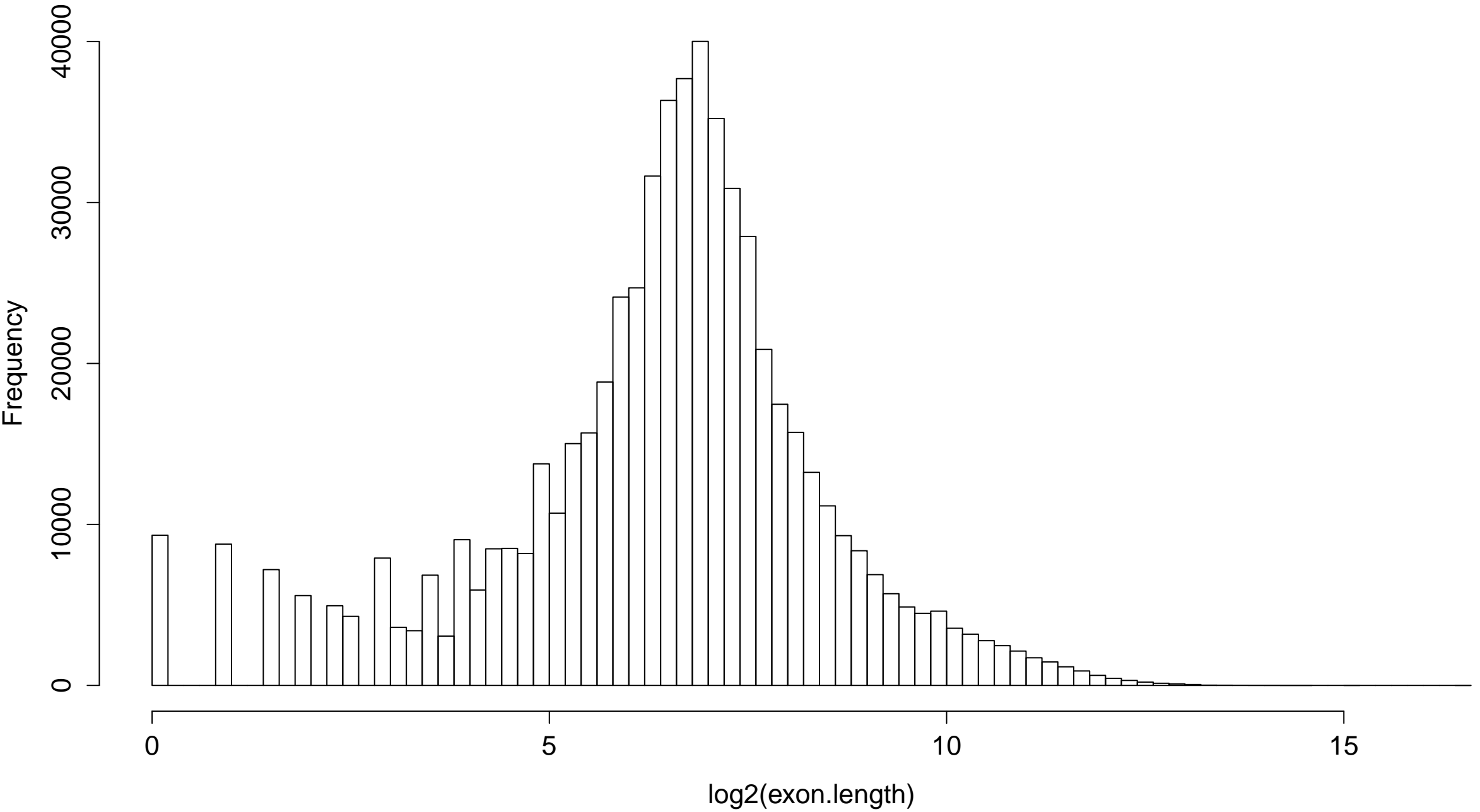
Histogram of \log_2(\text{exon.length})
