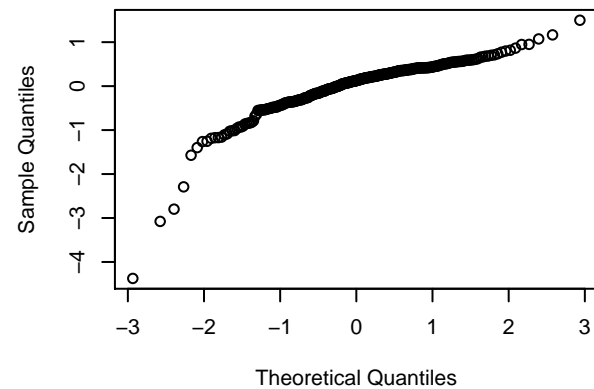
QQNORM 9
