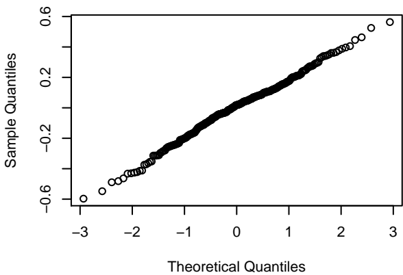
QQNORM 1
