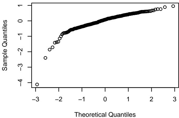
QQNORM 4
