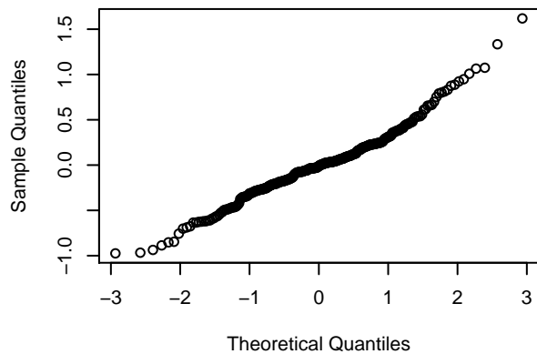
QQNORM 5
