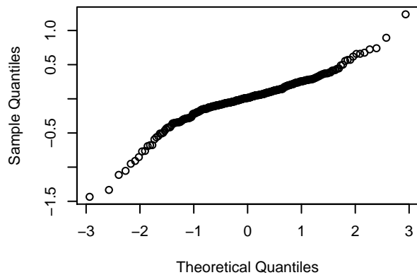
QQNORM 8
