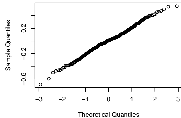
QQNORM 6
