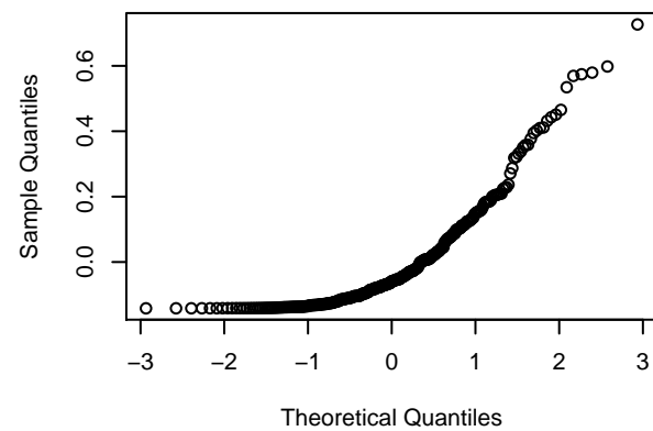
QQNORM 3
