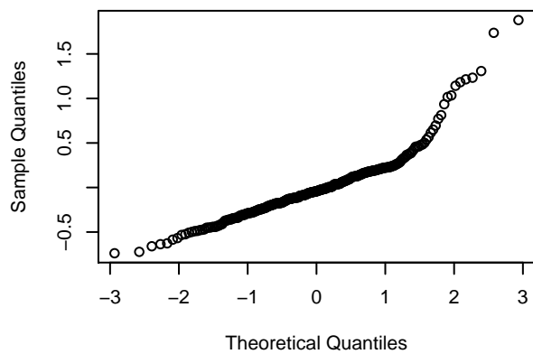
QQNORM 2
