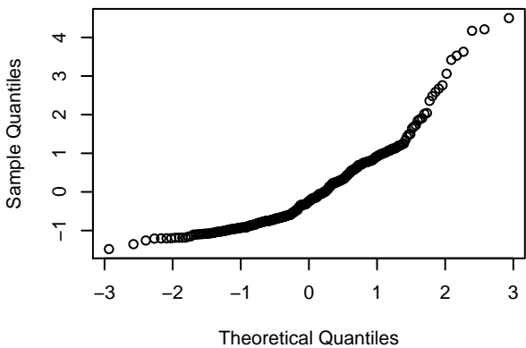
QQNORM 7
