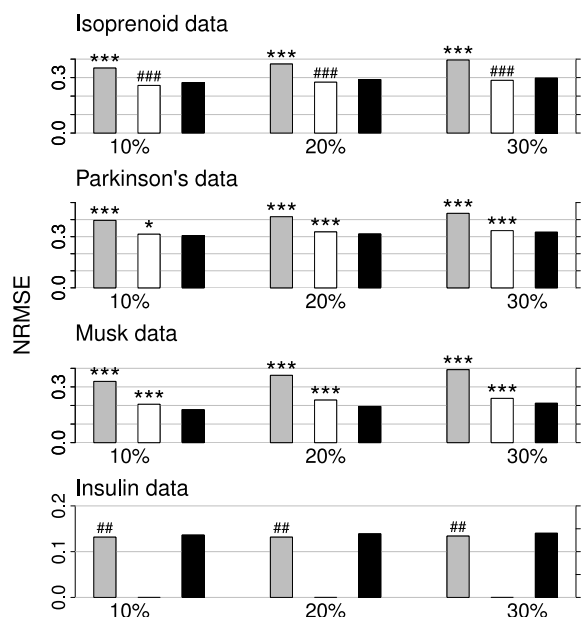
Fig. 1. Continuous data. Average NRMSE for KNNimpute (grey), MissPALasso (white) and missForest (black) on four different data sets and three different amounts of missing values, i.e., 10%, 20% and 30%. Standard errors are in the order of magnitude of 10^{-4} . Significance levels for the paired Wilcoxon tests in favour of missForest are encoded as “*” < 0.05 , “**” < 0.01 and “***” < 0.001 . If the average error of the compared method is smaller than that of missForest the significance level is encoded by a hash (#) instead of an asterisk. In the lowermost data set results for MissPALasso are missing due to the methods limited capability with regard to high dimensions.
