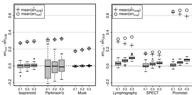
Fig. 4. Difference of true imputation error \text{err}_{\text{true}} and OOB imputation error estimate \widehat{\text{err}}_{\text{OOB}} for the continuous data sets (left) and the categorical data sets (right) and three different amounts of missing values, i.e., 0.1, 0.2 and 0.3. In each case the average \text{err}_{\text{true}} (circle) and the average \widehat{\text{err}}_{\text{OOB}} (plus) over all simulations is given.
