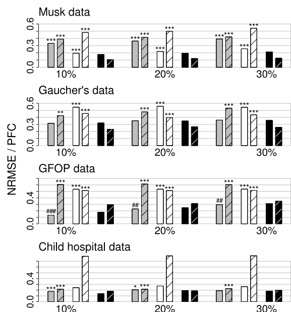
Fig. 3. Mixed-type data. Average NRMSE (left bar, shaded) for KNNimpute (grey), MICE (white) and missForest (black) on four different data sets and three different amounts of missing values, i.e., 10%, 20% and 30%. Standard errors are in the order of magnitude of 10^{-3} . Significance levels for the paired Wilcoxon tests in favour of missForest are encoded as “**” <0.05 , “***” <0.01 and “****” <0.001 . If the average error of the compared method is smaller than that of missForest the significance level is encoded by a hash (#) instead of an asterisk. Note that, due to ill-distribution and near dependence in the Child hospital data, the results for MICE have to be treated with caution (see Section 4.3).
