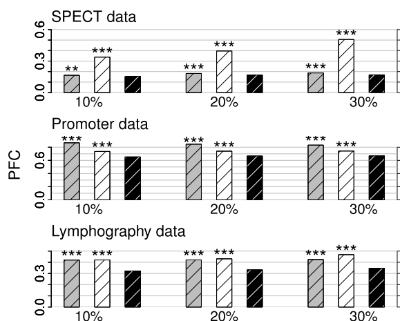
Fig. 2. Categorical data. Average PFC for cross-validated KNNimpute (grey), MICE (white) and missForest (black) on three different data sets and three different amounts of missing values, i.e., 10%, 20% and 30%. Standard errors are in the order of magnitude of 10^{-4} . Significance levels for the paired Wilcoxon tests in favour of missForest are encoded as “**” <0.05 , “***” <0.01 and “****” <0.001 .
