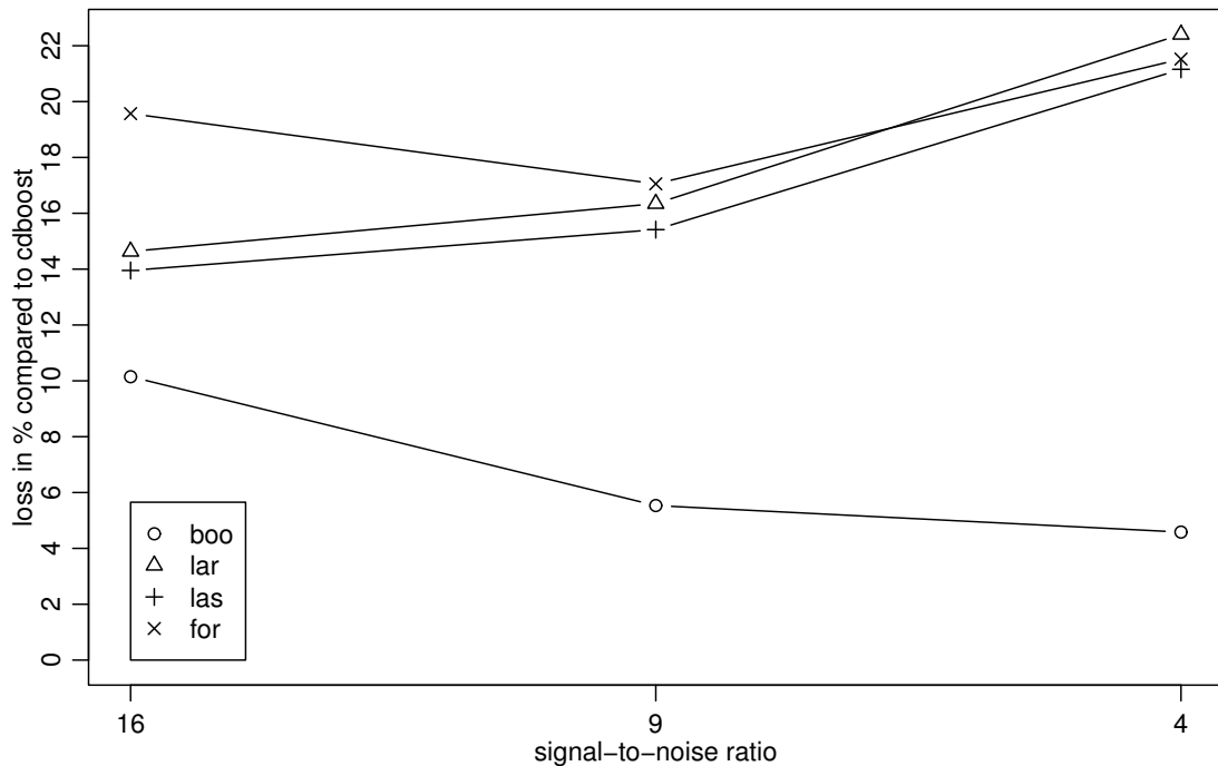
Figure 2: Percentage loss of the different methods (without forward stepwise variable selection) compared to CDBOOST for simulation model 2.
