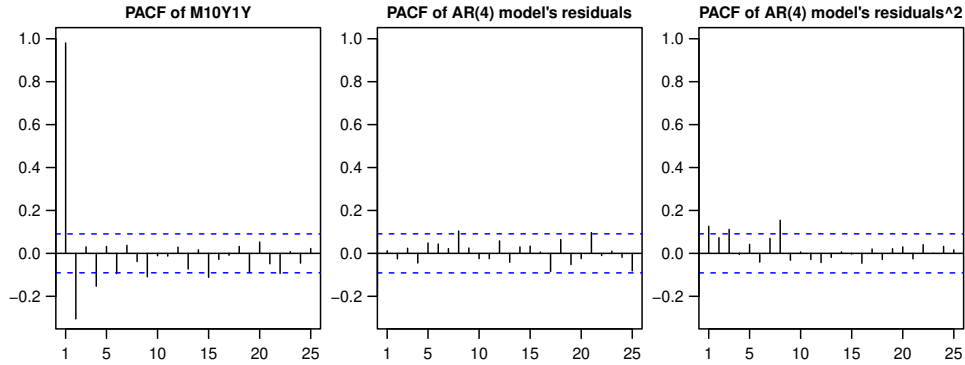
Figure 1: The sample partial autocorrelation function of the series M10Y1Y for the lags 1, \dots, 25 (on the left). The sample partial autocorrelation function of the Pearson residuals of a Gaussian AR(4) model (on the middle) and of the squared residuals (on the right) for the lags 1, \dots, 25 . The blue dashed lines are the 95% critical bounds for partial autocorrelation coefficients of an IID process.
