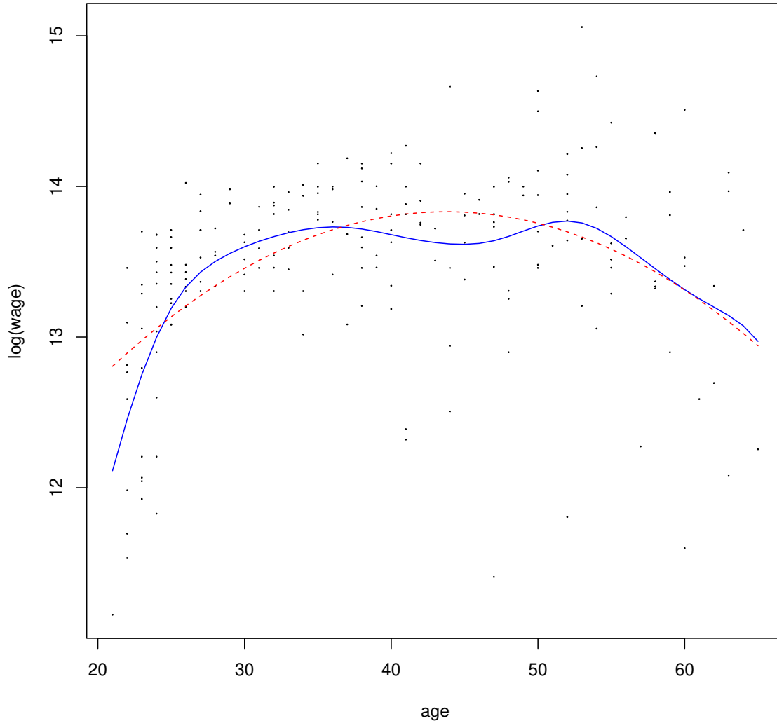
Figure 1: The figure on the upper left presents the parametric (quadratic, dashed line) and the nonparametric estimates (solid line) of the regression function for the cps71 data. The figure on the upper right presents the parametric (dashed line) and nonparametric estimates (solid line) of the gradient. The figures on the lower left and lower right present the nonparametric estimates of the regression function and gradient along with their variability bounds, respectively.
