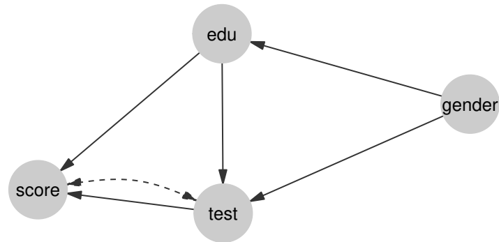
Figure 13: Visualization of the causal graphical model also shown in Figure 12, obtained when passing a confounding matrix indicating a bidirected edge between vertices test and score to fairadapt() . The resulting Semi-Markovian model can also be handled by fairadapt() , extending the basic Markovian formulation introduced in Section 2.3.
