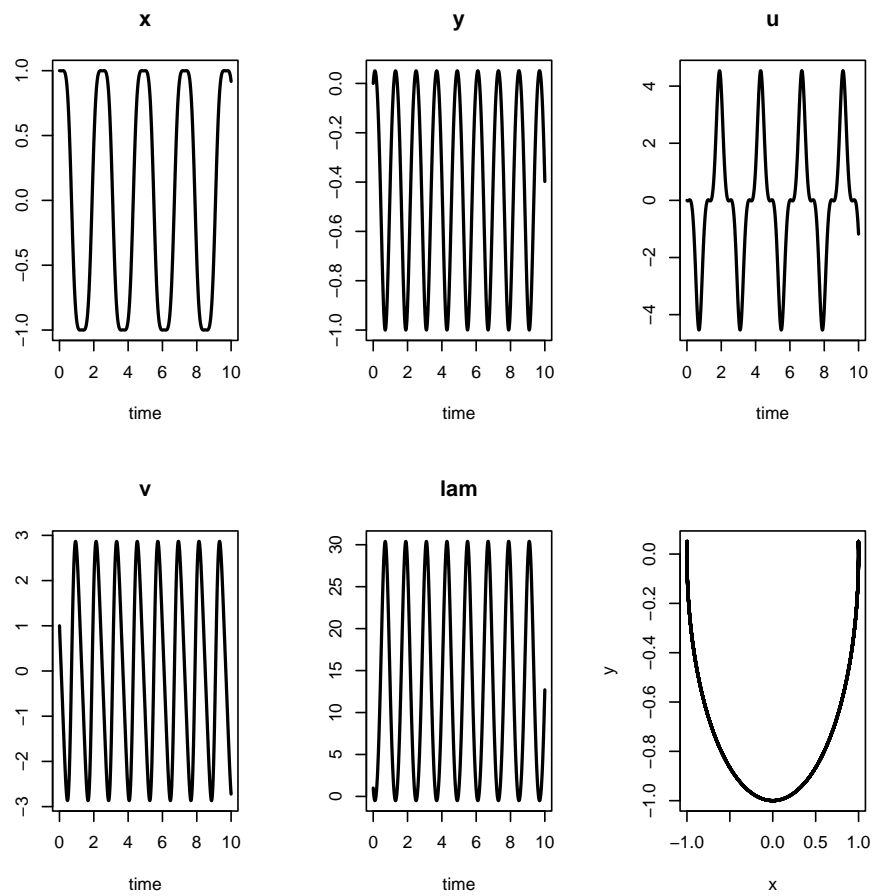
Figure 5: Solution of the pendulum problem, an index 3 differential algebraic equation using radau - see text for R-code
