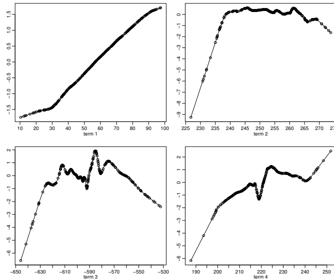
Figure 7.6: Four estimated ridge functions f_k(\cdot) from a projection pursuit fit to the ozone data ( \log(O3) \sim \cdot ).
