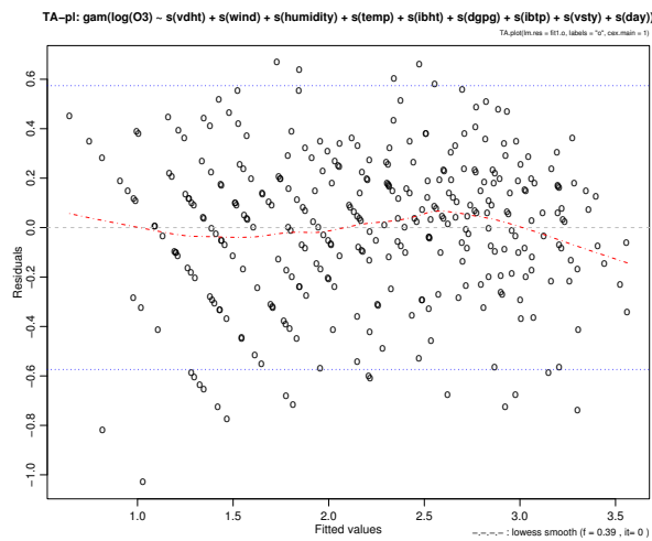
Figure 7.4: Estimated additive functions and Tukey-Anscombe plot for the ozone dataset with \log(O_3) as response variable and after omitting one outlier.
