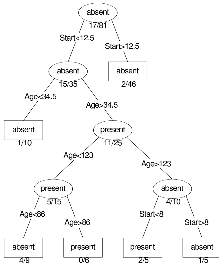
Figure 7.7: Classification tree for part of the kyphosis data set. Each node is labeled “presence” and “absence” (of kyphosis) according to majority vote, i.e., maximum likelihood. The ratios a/(a + b) are empirical misclassification rates, i.e., in this binary case, b = \#\{\text{cases with given level}\} , and a counts the other, “wrongly” labeled ones.
