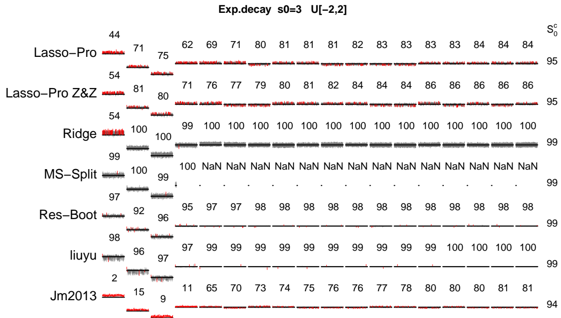
FIG 26. See caption of Figure 6 with the only differences being the size of the non-zero coefficients being U[-2, 2] and the design matrix type being Exp.decay .
