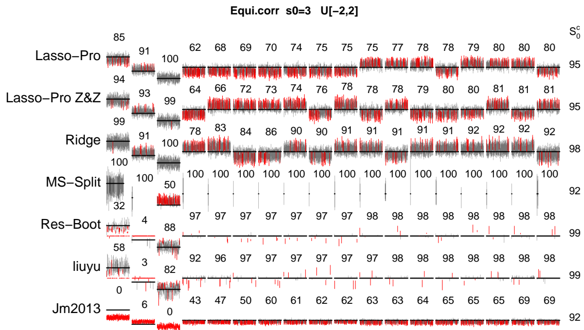
FIG 27. See caption of Figure 6 with the only differences being the size of the non-zero coefficients being U[-2, 2] and the design matrix type being Equi.corr .
