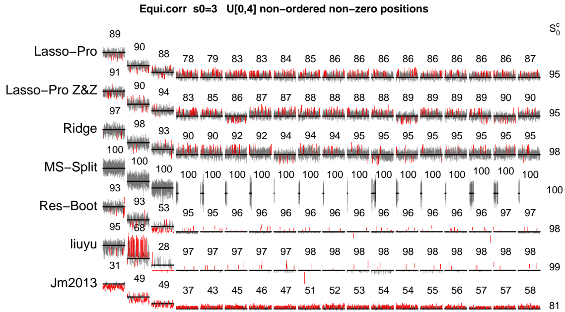
FIG 24. See caption of Figure 6 with the differences being the type of design matrix being Equi.corr , the size of the non-zero coefficients being U[0,4] and the positions of the non-zero coefficients being non-ordered (as in not the first s_0 columns of \mathbf{X} ).
