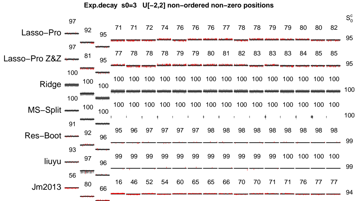
FIG 29. See caption of Figure 6 with the differences being the type of design matrix being Exp.decay , the size of the non-zero coefficients being U[-2, 2] and the positions of the non-zero coefficients being non-ordered (as in not the first s_0 columns of \mathbf{X} ).
